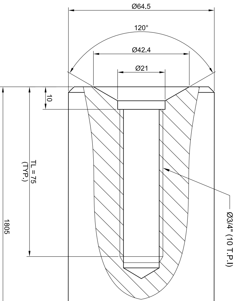
DETAIL - A (SCALE - 1:1)
