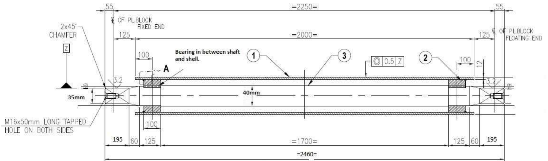
Roller for lifting of conveyor
