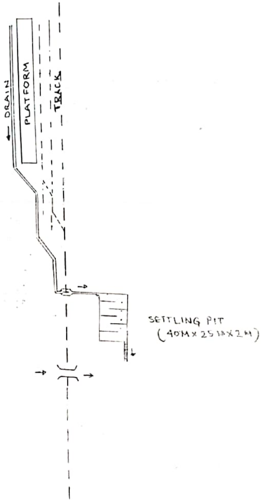
LAY OUT PLAN OF COAL SETTLING PIT AT MANOHARPUR Yard
