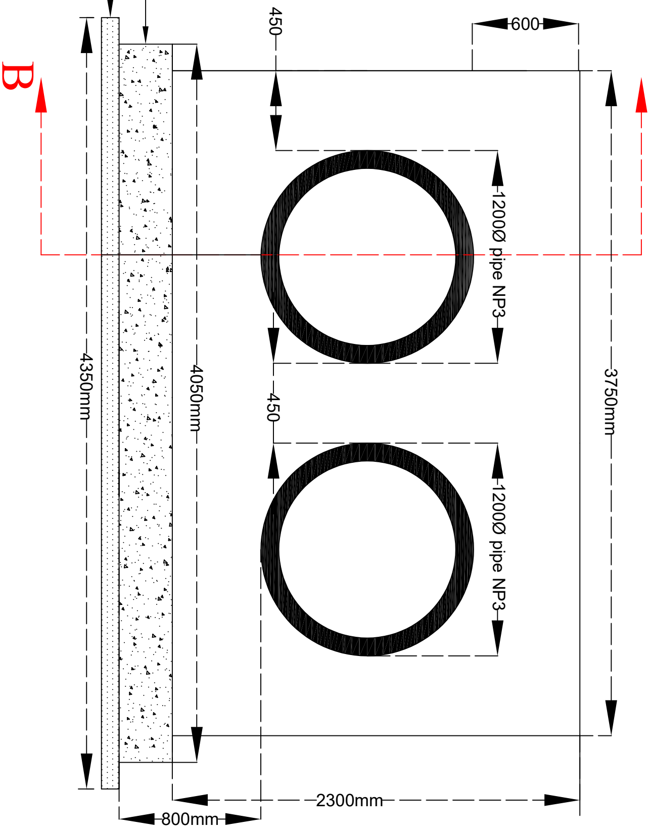
FIGURE 2: SECTION A - A
