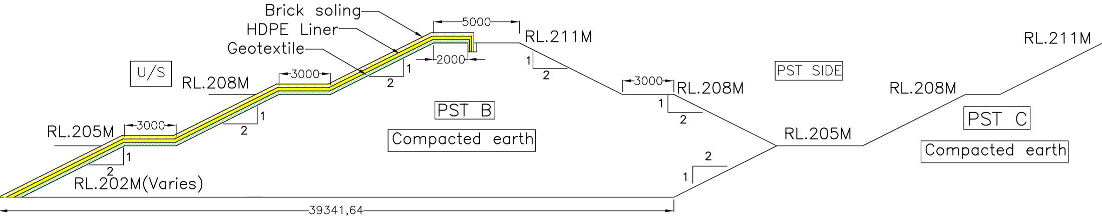
SECTION 2-2: Cross section of PST B (PST C SIDE)
