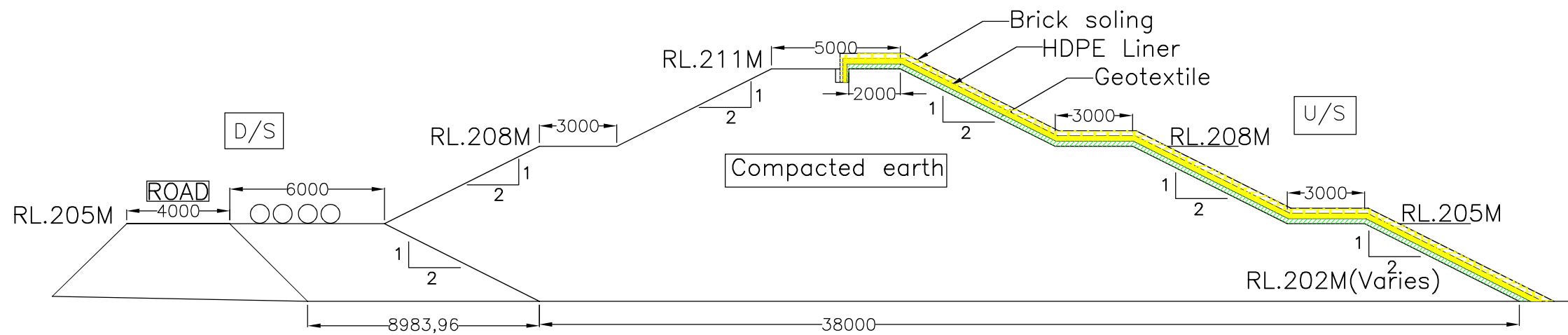
SECTION 1-1: Cross section of PST B (Reservoir side)
