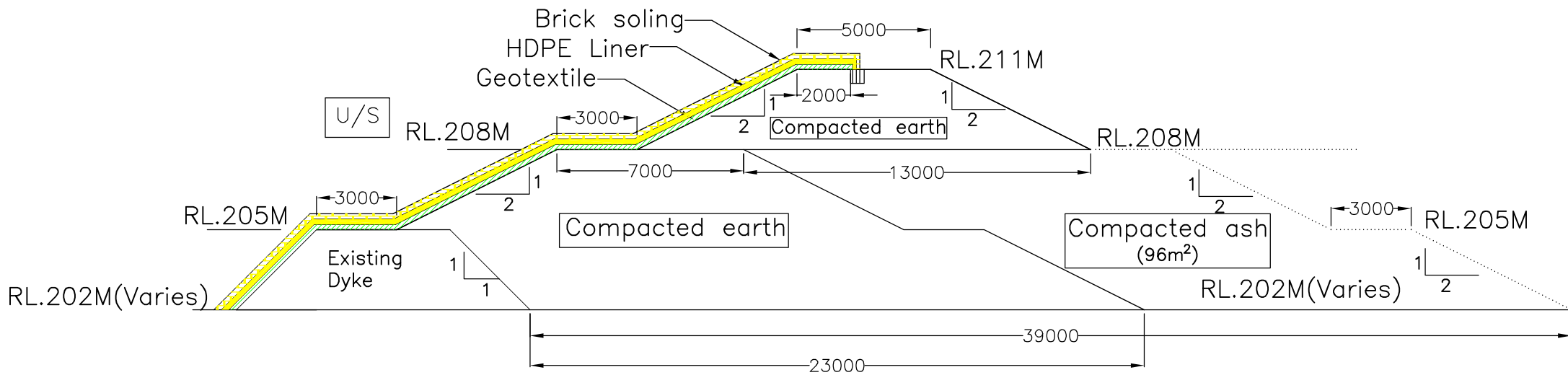
SECTION 3-3: Cross section of PST B (POND B SIDE) ALTERNATIVE II
